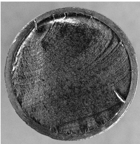
Figure 7. Beach marks on the fracture surface are clear signs that this stud from the right rear of a van failed from fatigue. Failure was less than 121 days since installation.
