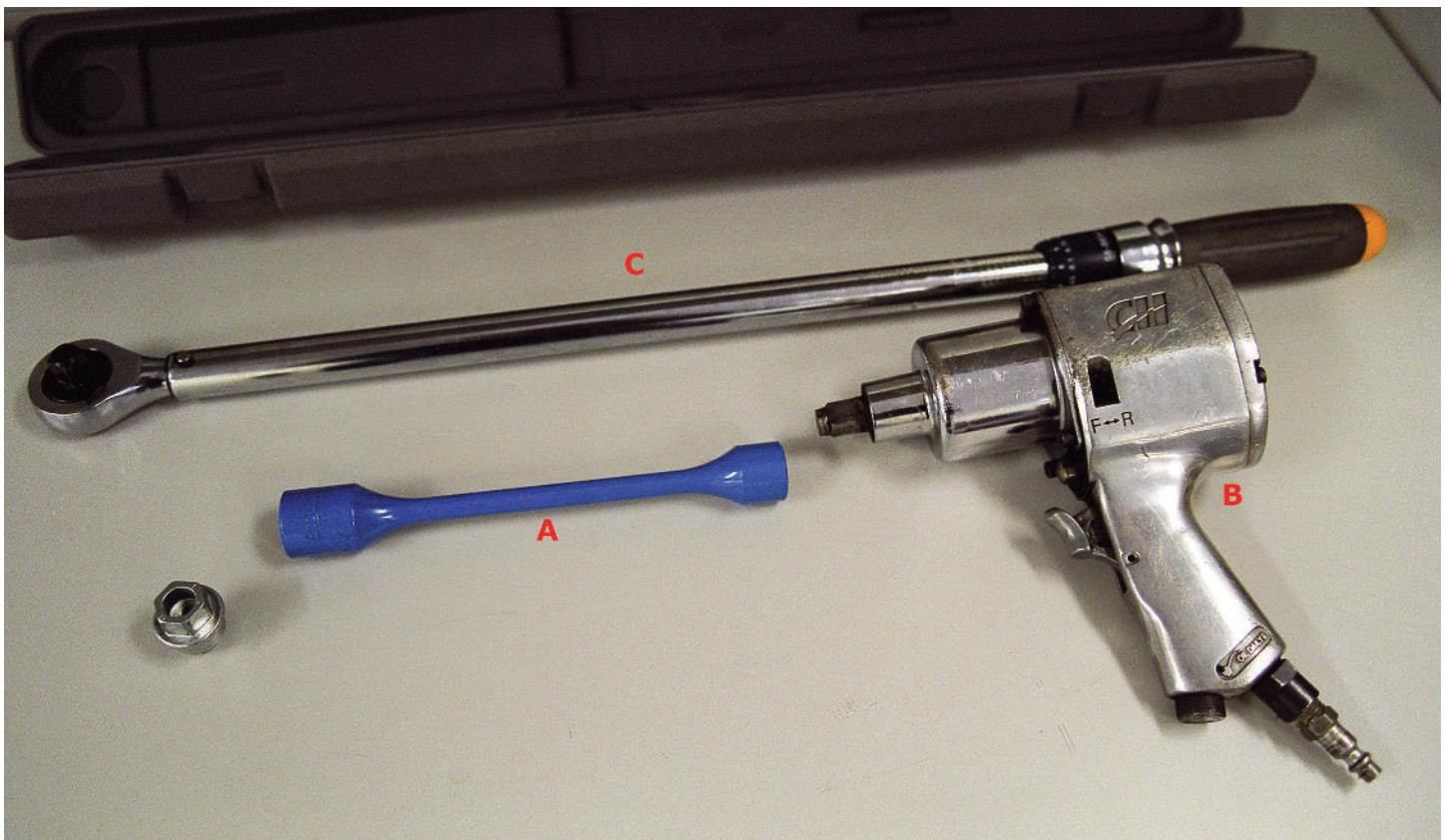
Figure 8. A: an 80 foot-pound Torq Stik. B: air wrench that Torq Stik attaches to. C: A manual torque wrench.
